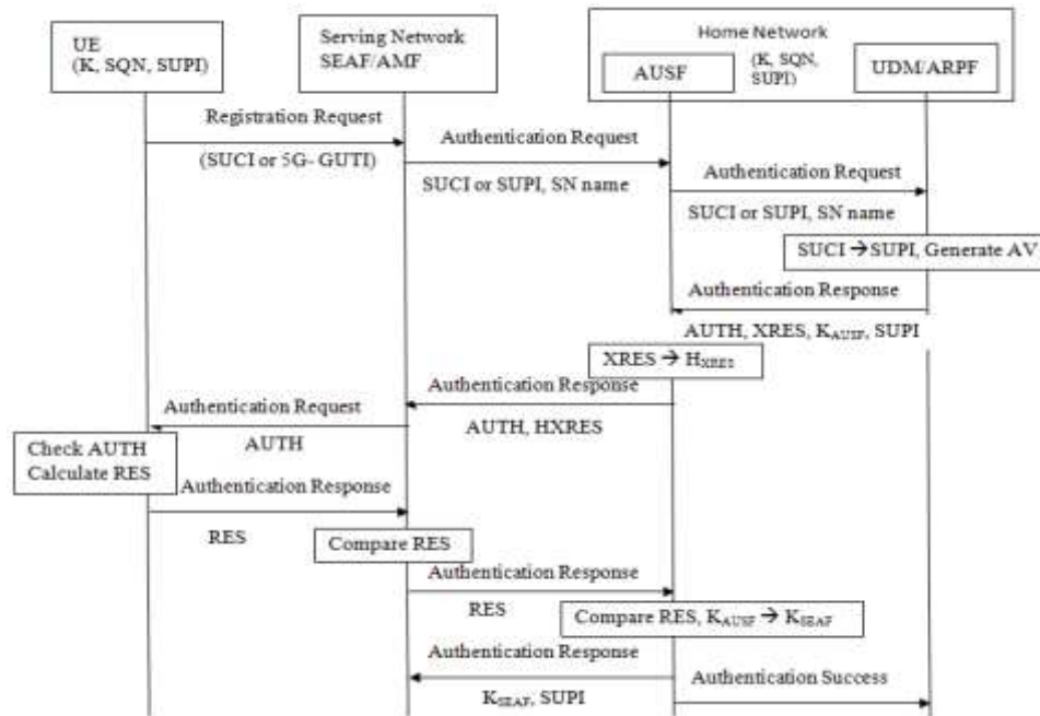
Figure 4: 3GPP 5G-AKA
