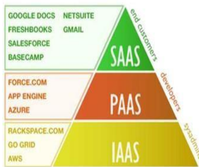
Fig.1 Cloud Services
