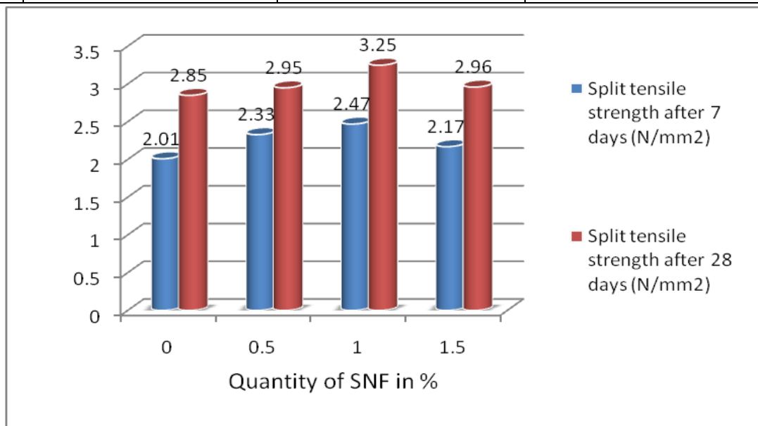
Graph-2 Test Results of Split Tensile Strength of All The Mixes Prepared With Variable Quantity of Superplasticizer
