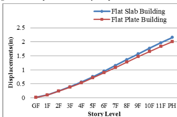
Figure 9. Comparison of Story Displacement in Y-Direction
