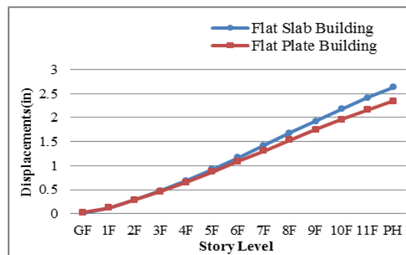
Figure 8. Comparison of Story Displacement in X-Direction
