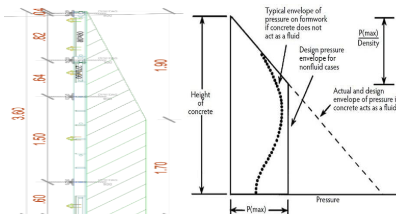
Figure Error! No text of specified style in document..3: Pressure Diagram
