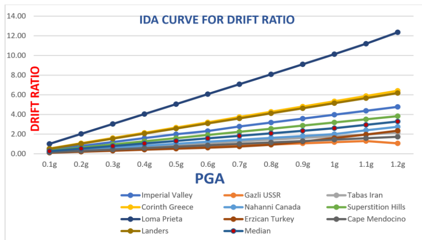
Figure 2: Drift ratio IDA curve
