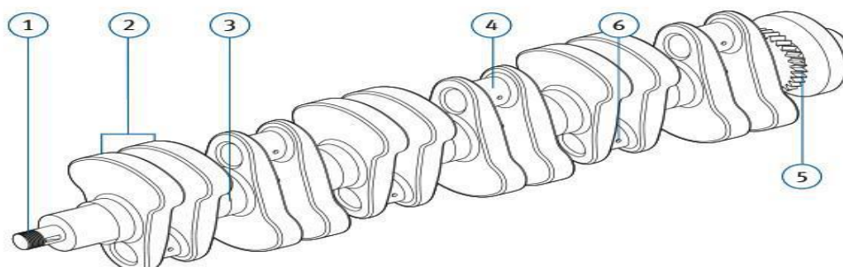
Fig.1 Crankshaft Nomenclature
