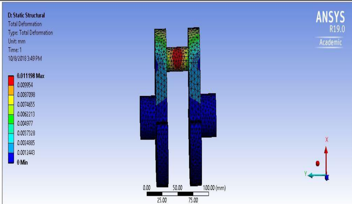
Fig.2 Total deformation in Case-1 for model 1
