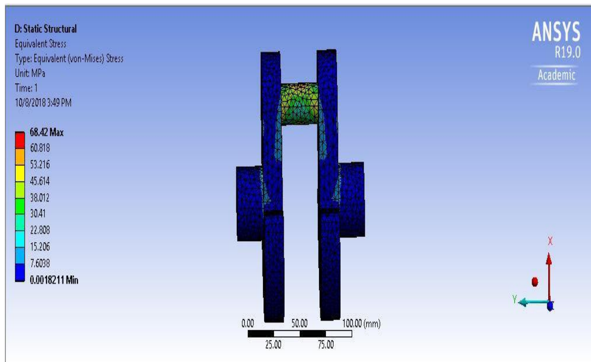
Fig.3 Equivalent stress in Case-1 for model 1
