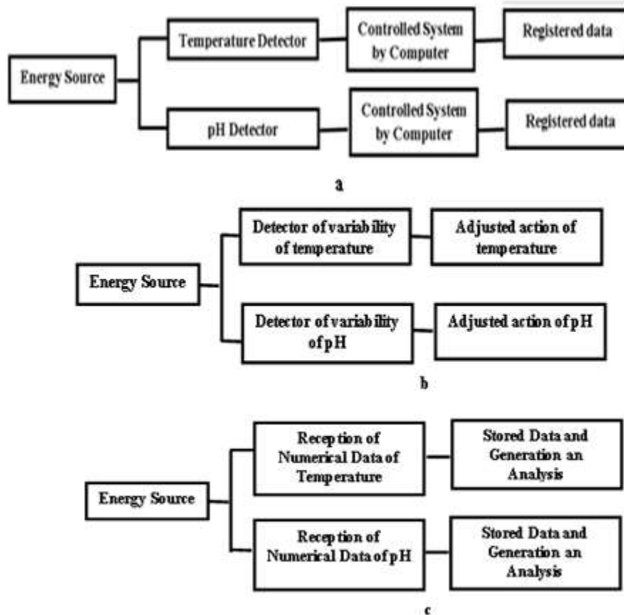
Figure 4 Automatization system to control physicochemical factors constituted by (a) Principal system, (b) Adjusted System and (c) Registration data values
