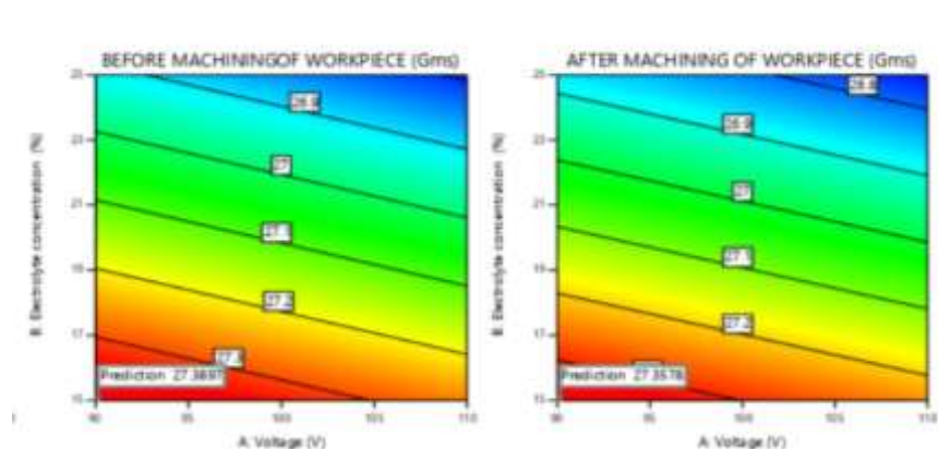
Figure 4 Before machining and after machining of work piece with respect to Voltage and Electrolyte concentration. The relationship between the voltage and the Electrolyte concentration is displayed in this tool wear contour plot. The peak value of the value is then displayed as a function of the variables, and the voltage hold limits were 110v. The relationship between the voltage and the electrolyte concentration can be seen in this material removal contour map shows the predication after machining is 0.107.
