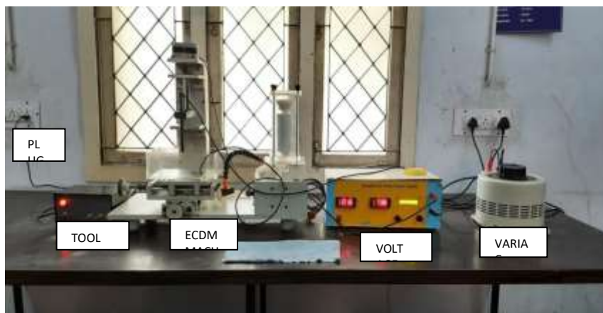
Fig 1 (ECDM setup)
