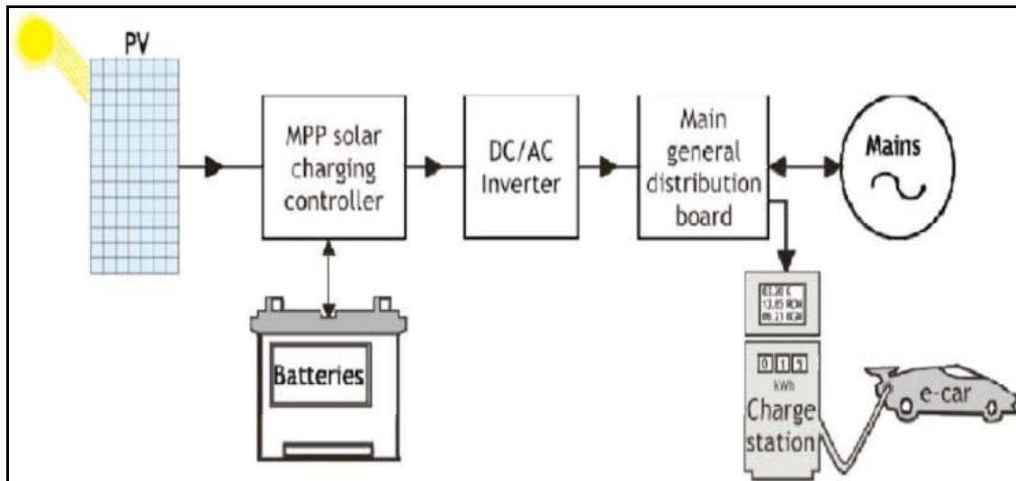
Fig.1 Block Diagram of EV charging station by using solar panel
