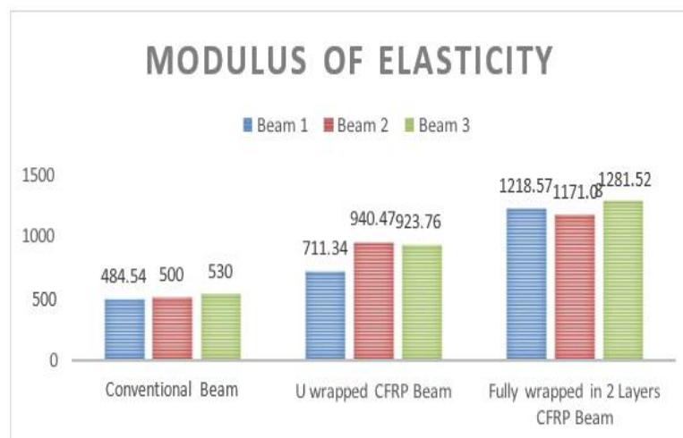
Fig 16. Modulus of Elasticity graph of beams
