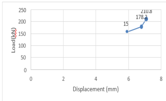
Fig 11. Load vs Displacement graph of U- shaped wrapped RC beam
