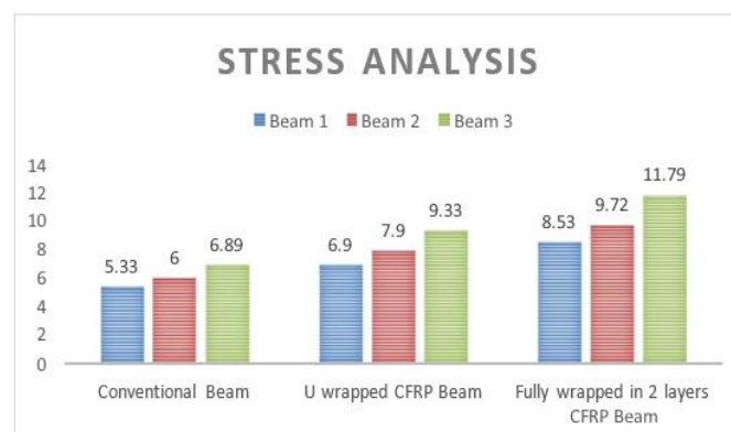
Fig 14. Stress Analysis of beams
