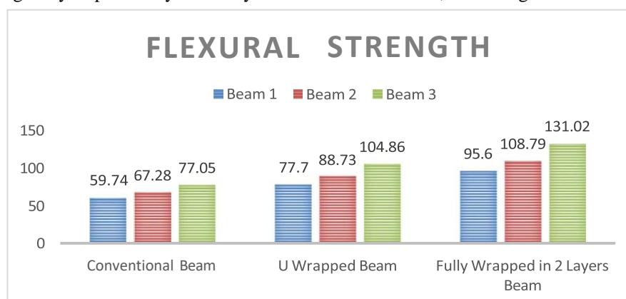
Fig 13. Flexural Strength graph of beams
