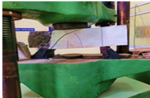
Fig 17. Crack propagation in control beam
