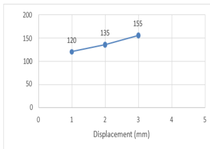
Fig 10. Load vs Displacement graph of conventional beam
