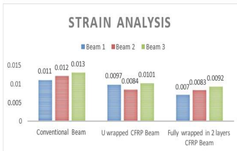
Fig 15. Strain Analysis of beams
