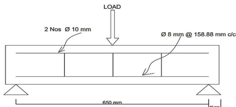
Fig 3- Reinforcement details of Beam
