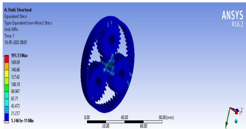
Figure 10 Von-misses stress at 3500 Rpm of 15 Ni 5Cr4Mo1 Material
