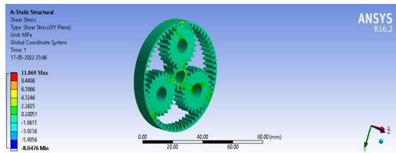
Figure 20 Shear stress at 3500 Rpm of AL 7075 Material
