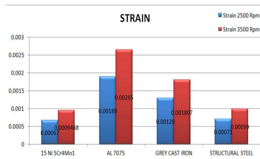
Figure 36 Strain graph
