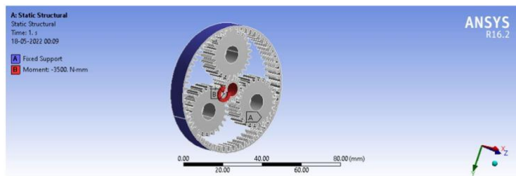
Figure 4 RPM 3500
