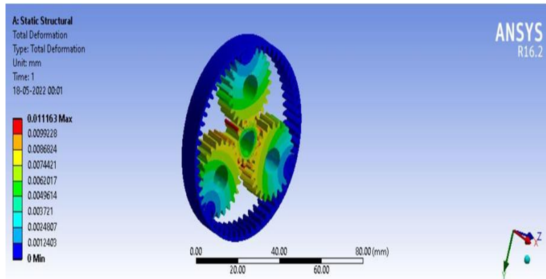
Figure 11 Total deformation at 3500 Rpm of 15 Ni 5Cr4Mo1 Material
