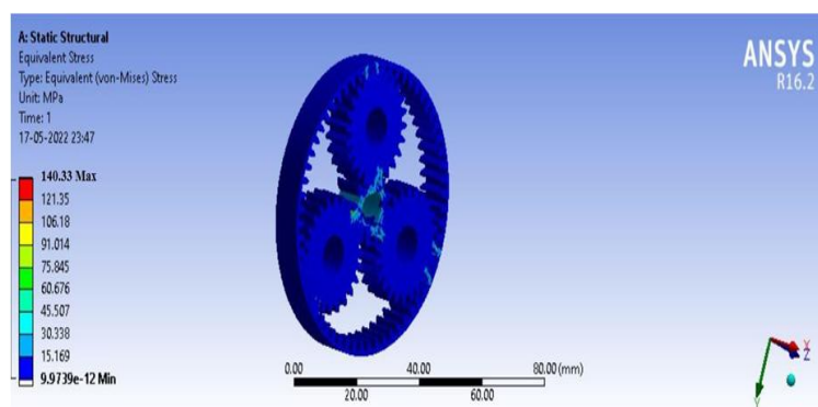
Figure 14 Von-misses stresz at 2500 Rpm of AL 7075 Material
