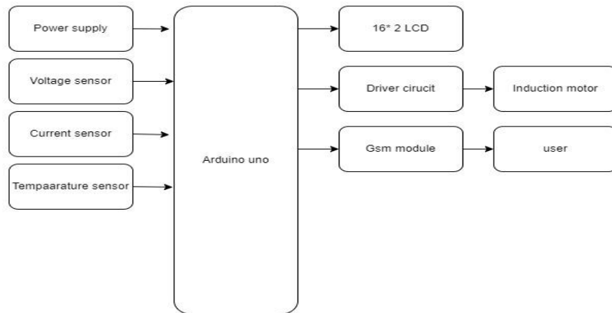
FIG:1- Proposed System Block Diagram
