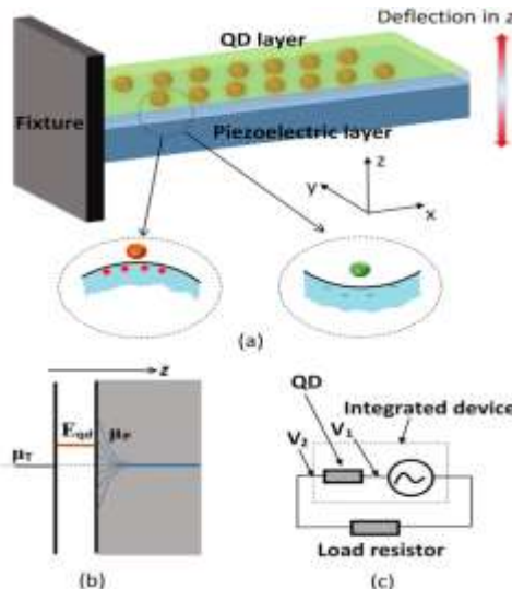
Figure 2: Piezoelectric Layers
