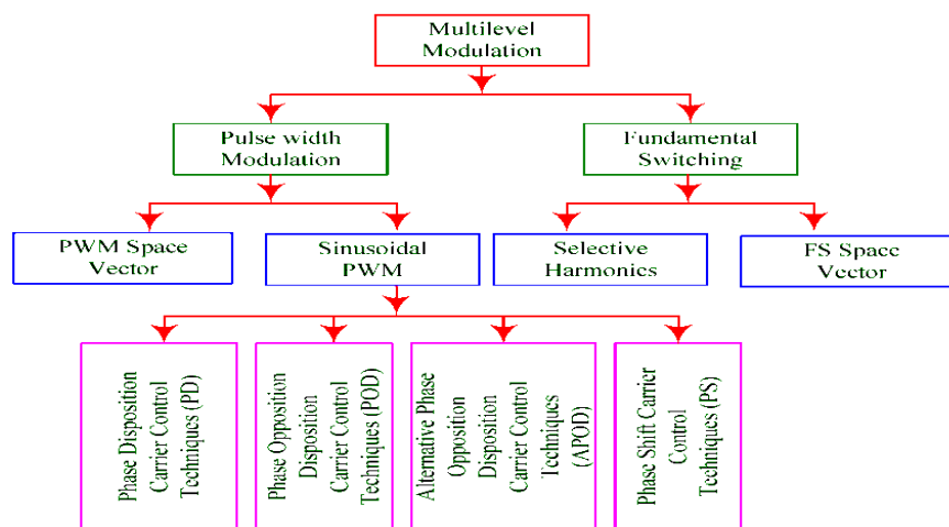
Figure 4: Modulation Strategies
