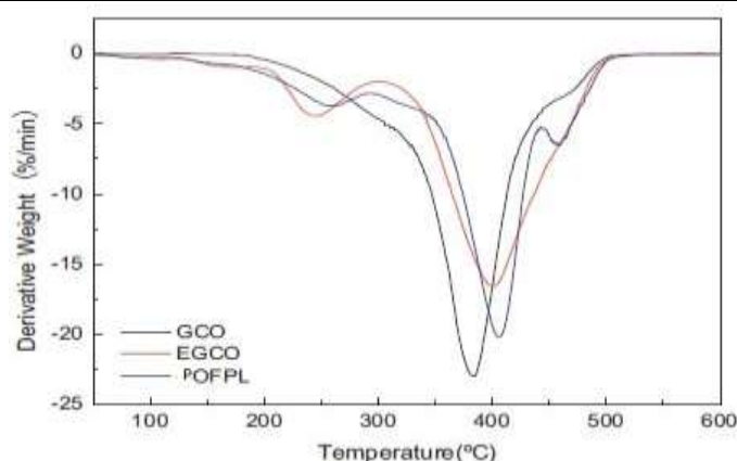
Fig. 9. DTG curves of GCO, EGCO and POFPL.
