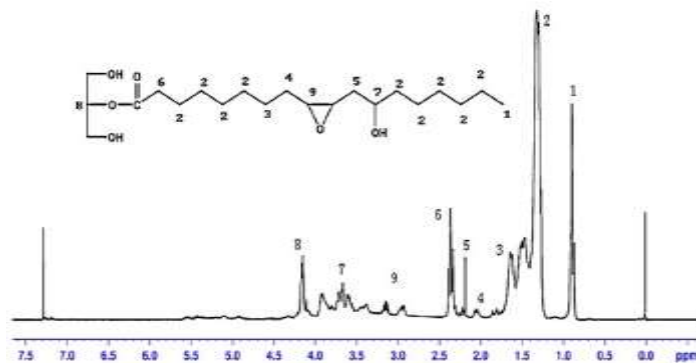
Fig. 6. 1 H NMR spectra of EGCO
