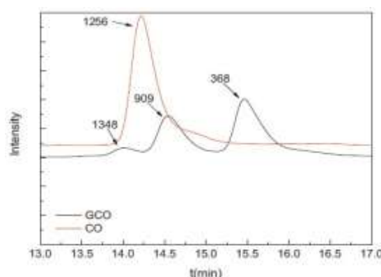
Fig. 4. The GPC spectra of palm oil and GCO.
