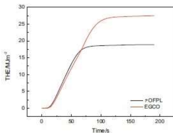
Fig. 13. Total heat evolved (THE) for GCO filled PU foam, POFPL filled PU foam.
