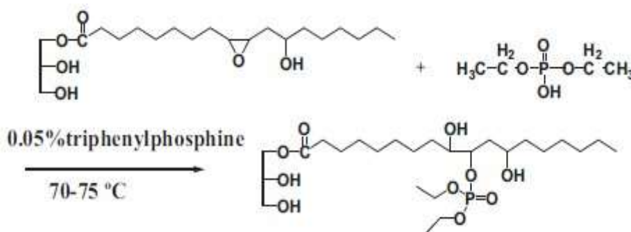
Fig. 2. The chemical reaction between EGCO and diethyl phosphate.
