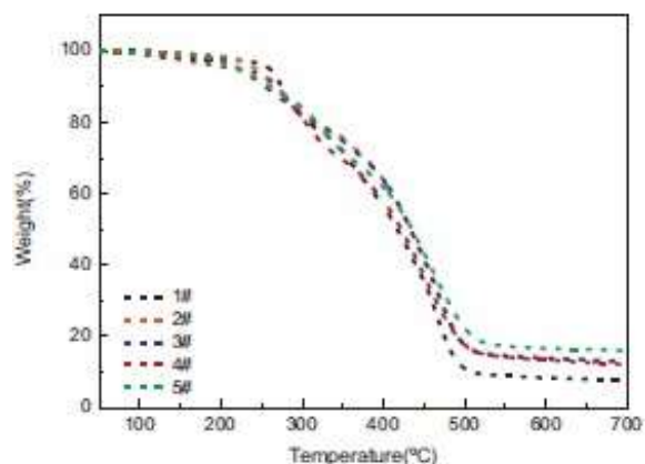
Fig. 14. TGA curves of polyurethane foams.
