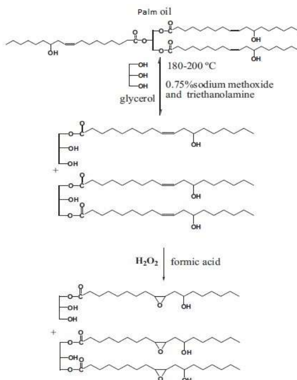
Fig. 1. The alcoholysis reaction and epoxidation reaction of palm oil.
