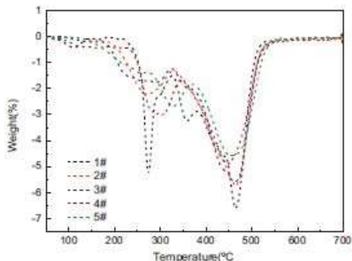
Fig. 15. DTG curves of polyurethane foams.
