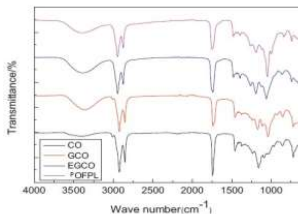
Fig. 3. FT-IR spectra of palm oil, GCO, EGCO and POFPL.
