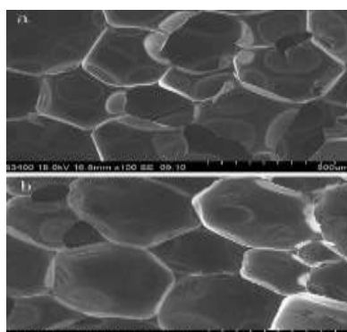
Fig. 10. SEM micrograph for PU foam prepared from GCO (a). SEM micrograph for PU foam prepared from POFPL (b).
