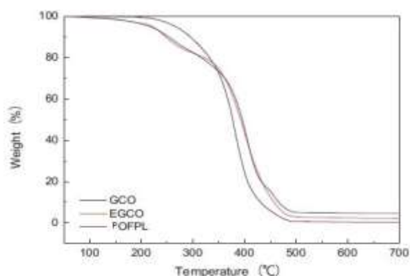
Fig. 8. TGA curves of GCO, EGCO and POFPL.
