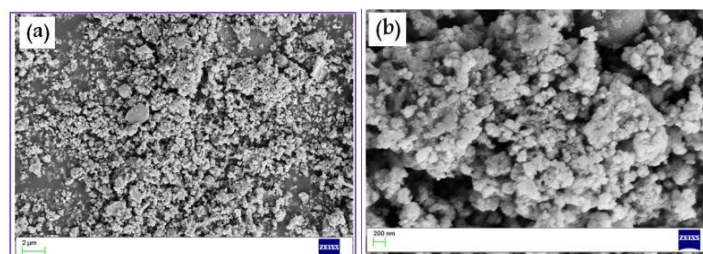
Figure 2 : FESEM images of \text{MoO}_3 nanoparticles at (a) – low magnification and (b)- high magnification
