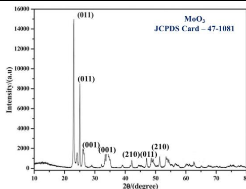
Figure 1: PXRD pattern of synthesized \text{MoO}_3 nanoparticles
