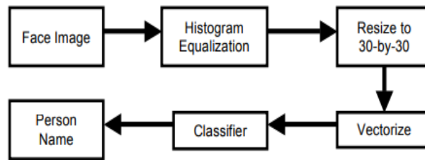
Fig3.4: Face recognition algorithm
