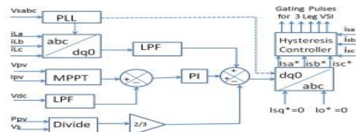
Fig. 2. Control for shunt compensator.
