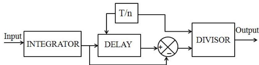
Fig. 2. Block diagram representation of MAF
