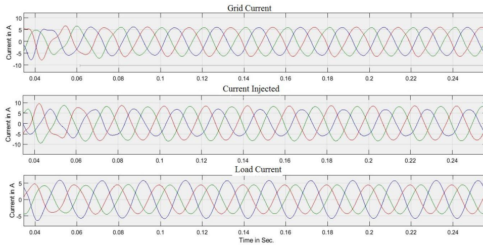
Fig. 7. Current compensation waveforms
