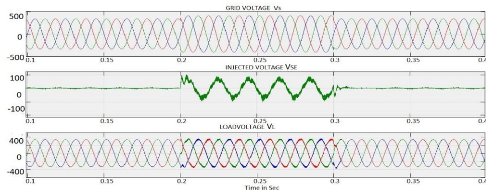
Fig. 8. Voltage compensation waveforms a)input grid voltage: 0.2pu swell is applied between 0.2sec and 0.3 sec b) Compensating voltage injected from VSC phase A c) Improved load voltage
