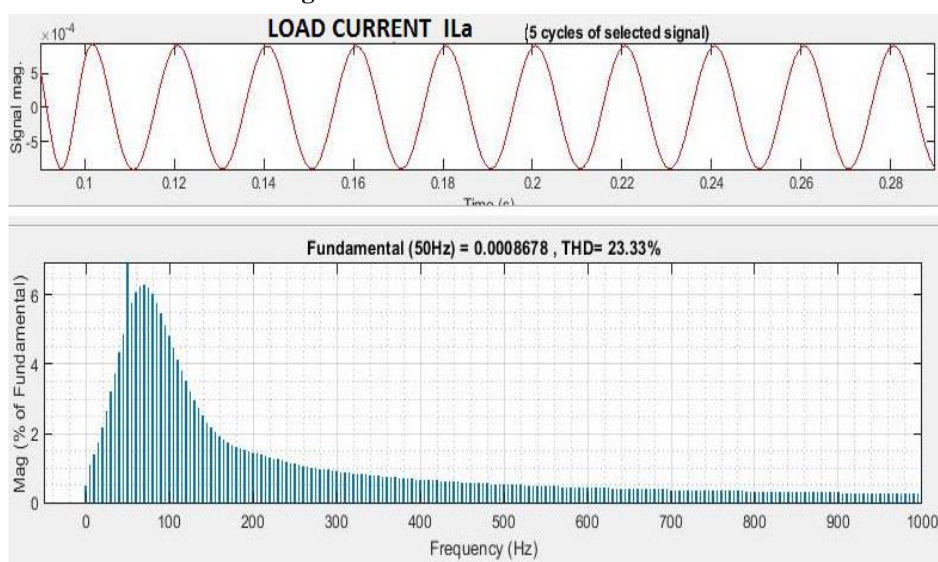
Fig. 11. Load current THD = 23.33%
