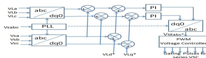
Fig. 3. Control for series compensator
