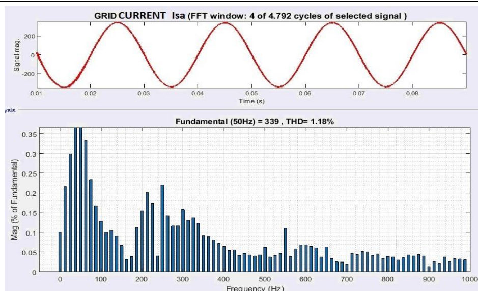
Fig. 10. Grid Current THD = 1.18 %
