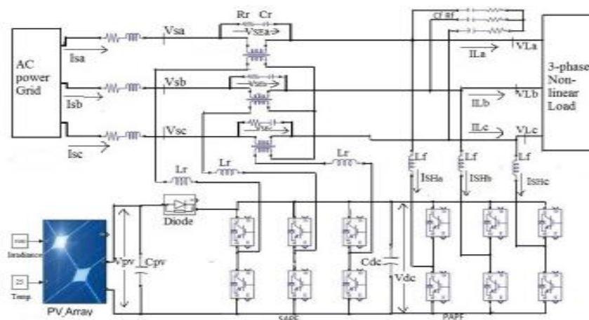
Fig. 1. Basic Topology
