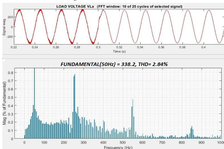
Fig. 12. Load Voltage THD = 2.84%
