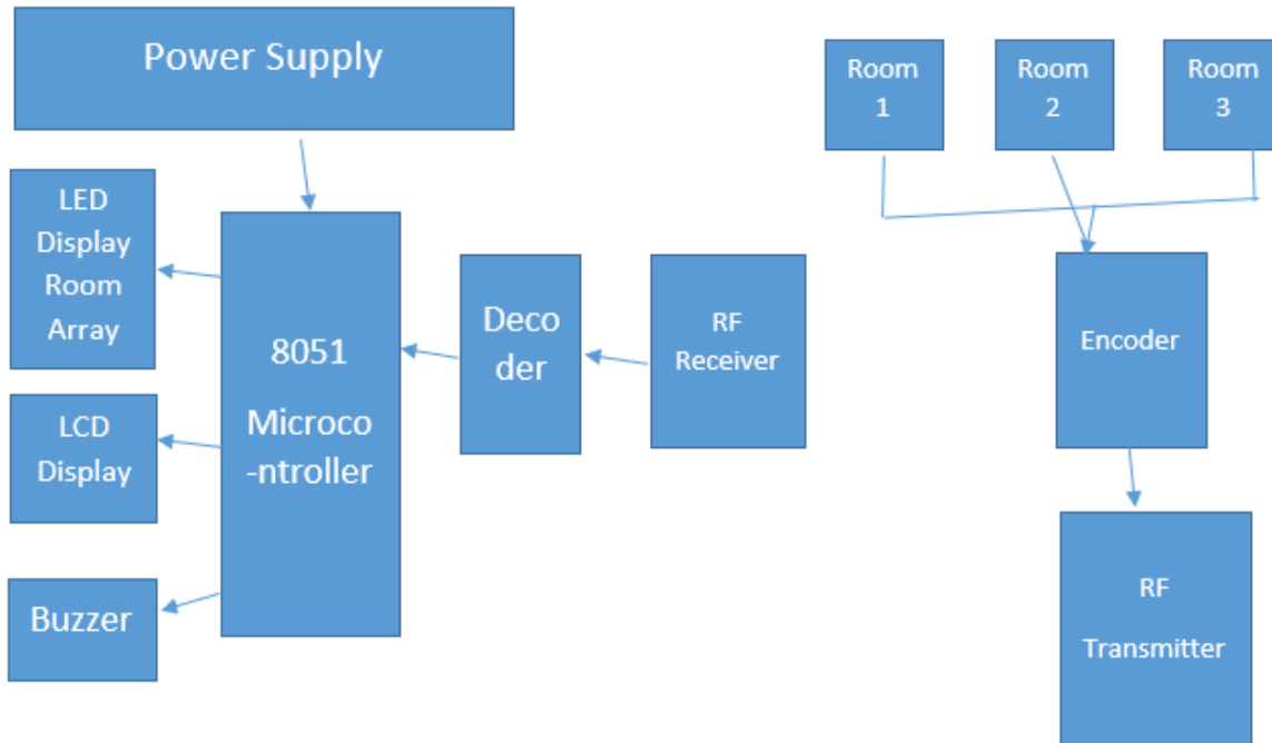
Figure 1: Block Diagram
