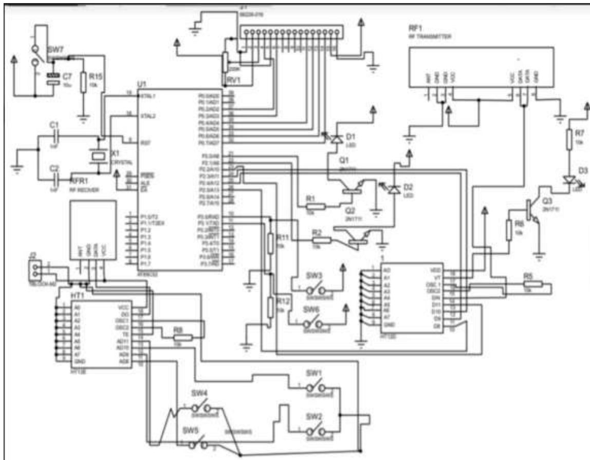
Figure 2: Circuit Diagram
