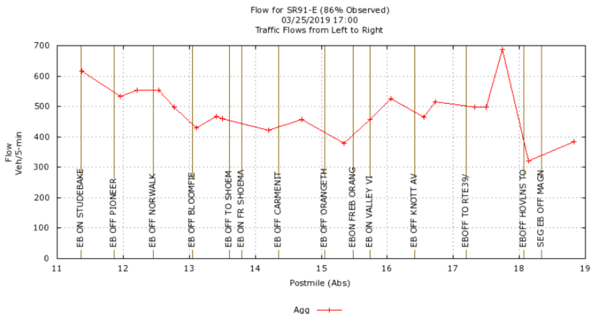
FIGURE 4 Traffic Flow Graphic for SR91-E
