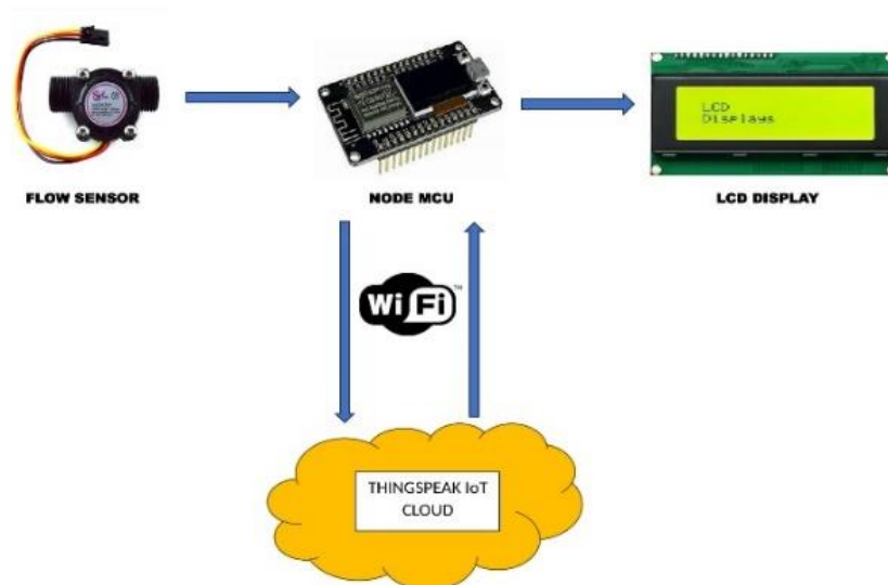
Fig.1 Block diagram of water leakage detection system
