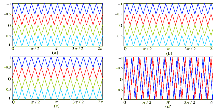
Figure 5: Carrier arrangements of (a) phase disposition (PD); (b) phase opposition disposition (POD); (c) alternative phase opposition disposition (APOD); and (d) phase shifted (PS) techniques.
