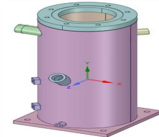
Fig.4 3D model and a graphical representation of a standard air-oil separator
