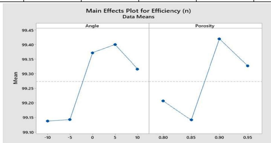
Fig.5 Main effects plot for efficiency
