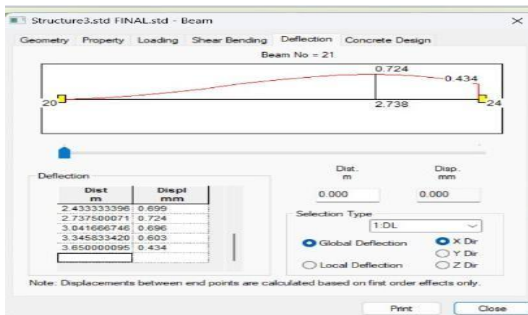
STRESS GRAPHS
