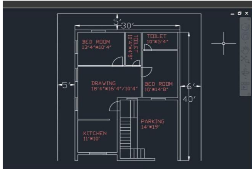
Fig 2. Dimensions of the building
