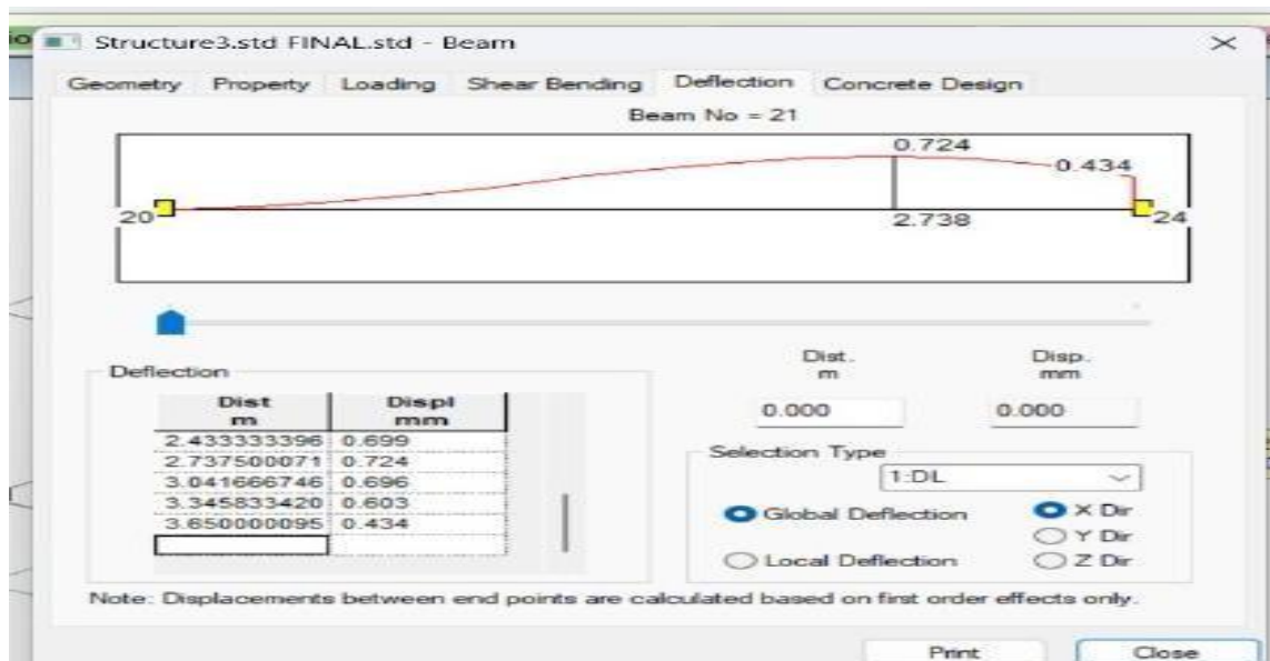
BEAM DEFLECTION
