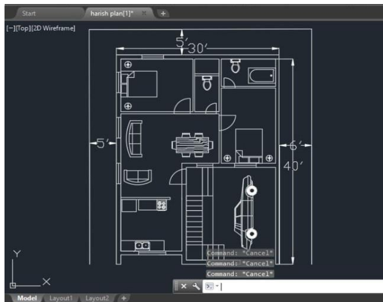
Fig 1. Plan of residential building
