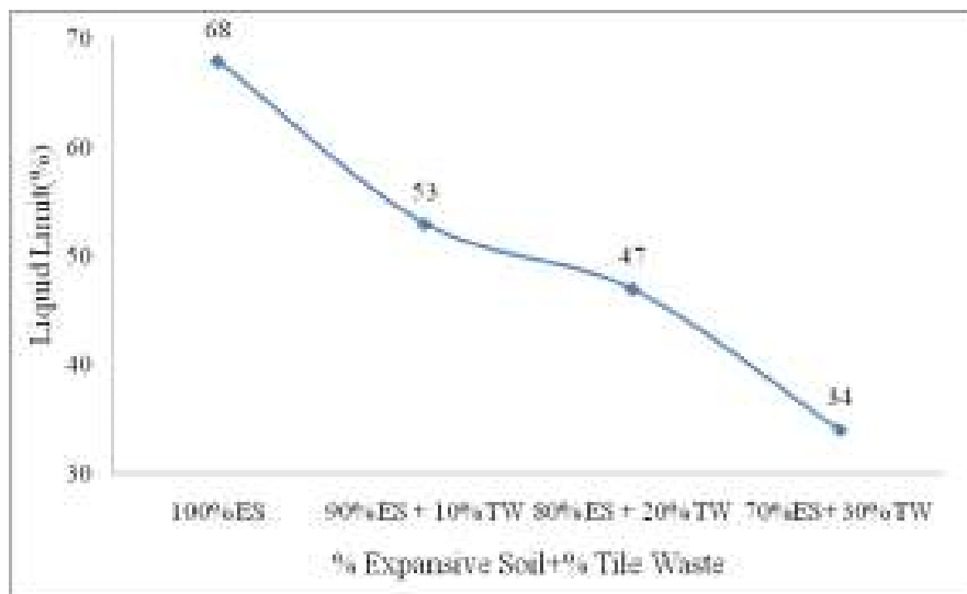
Variation of Liquid limit with percentage of Tile Waste
