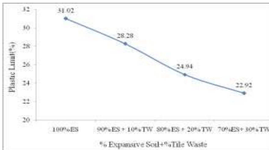
Variation of Plastic Limit with Percentage of Tile Waste
