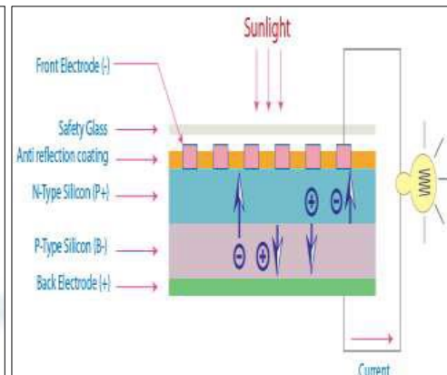
Fig.2. Photovoltaic Effect.
