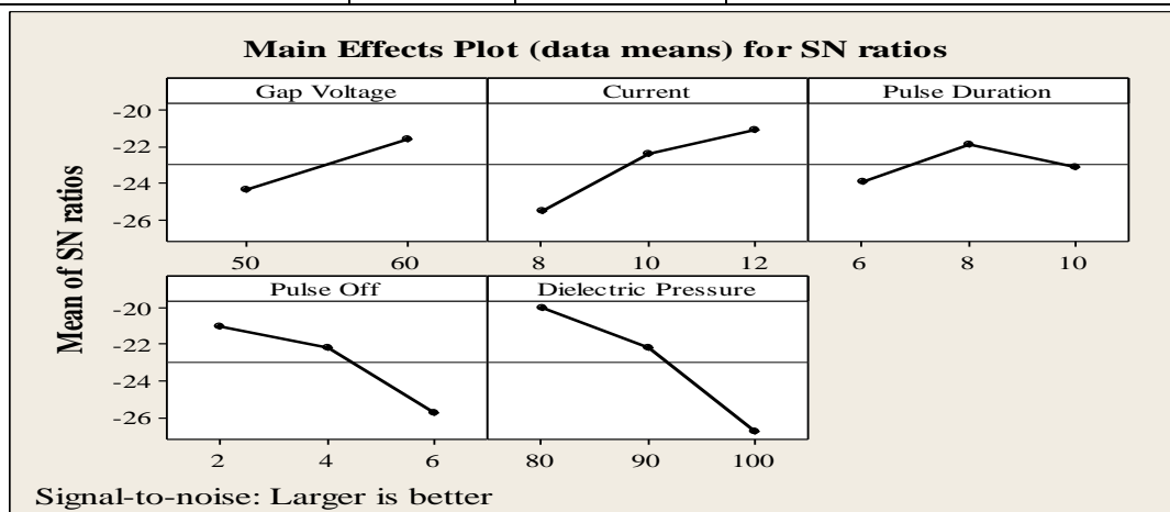
Fig.2 SNR plot for MRR
