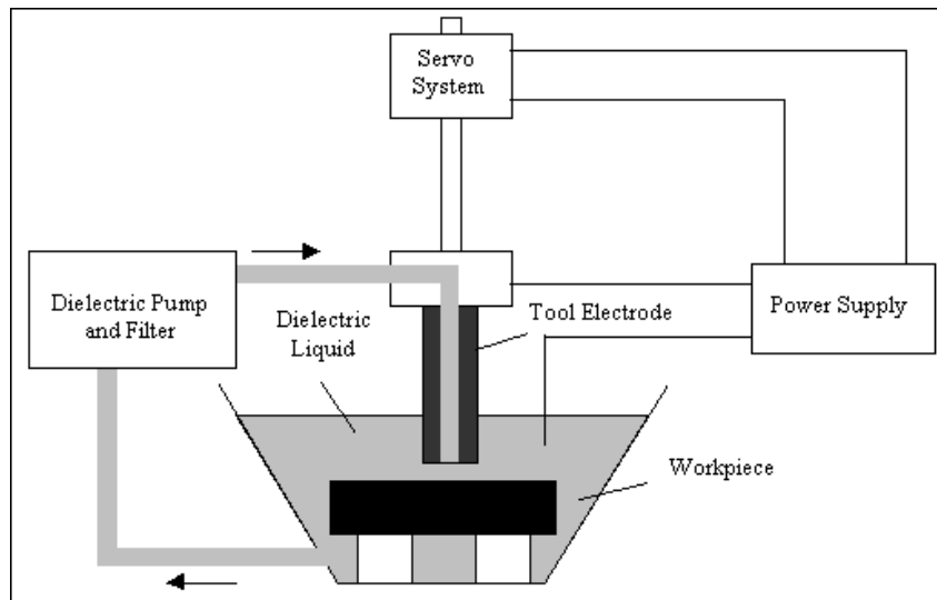
Fig. 1 Setup of EDM Process
