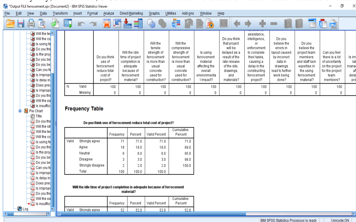
Figure 6 : Output File
