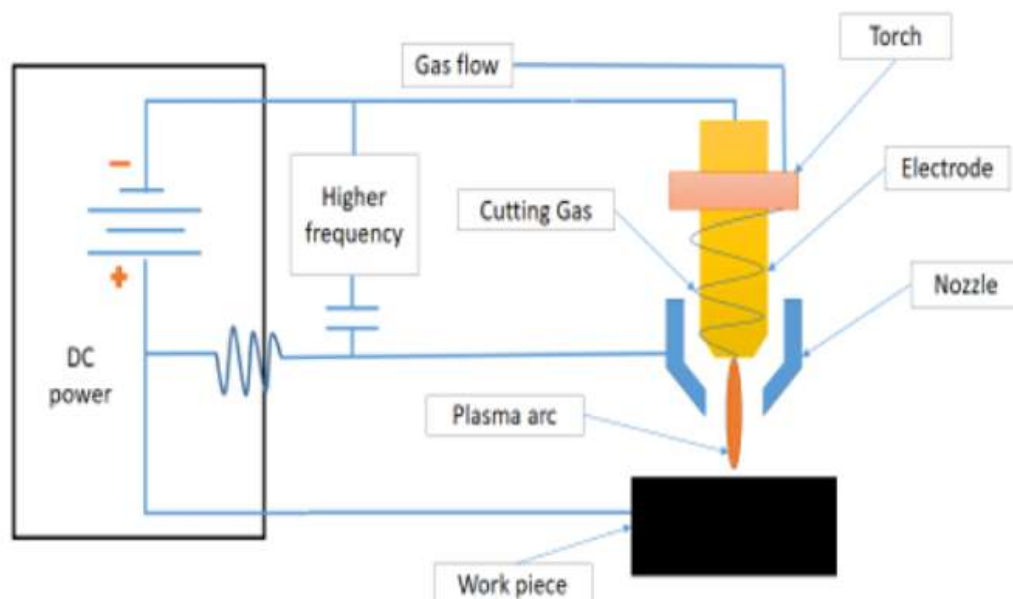
Fig. 1: Schematic diagram of plasma arc cutting
