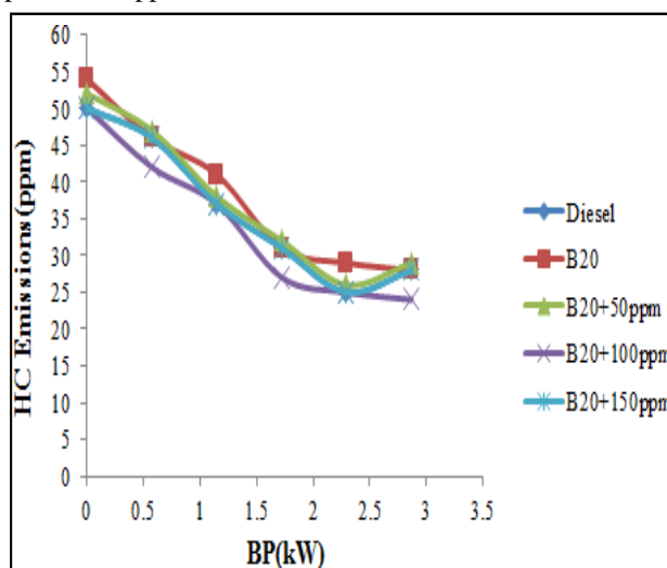
Figure 4. Variation of HC Emissions with B.P
