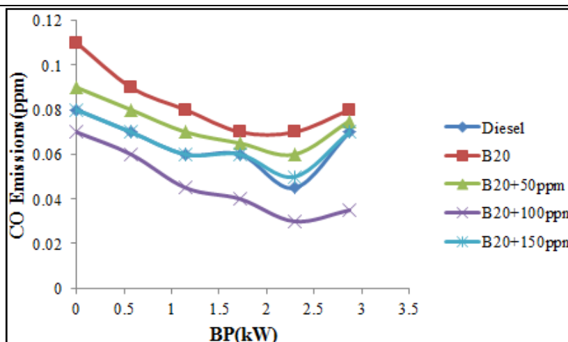
Figure 5. Variation of CO Emissions with B.P
