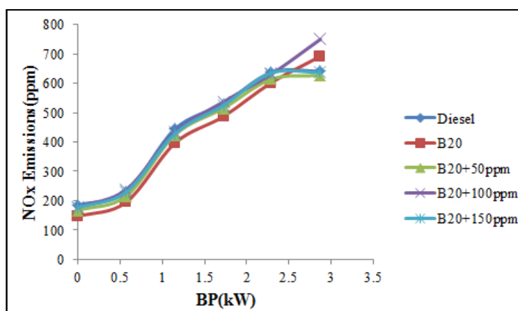
Figure 6. Variation of NO x Emissions with B.P
