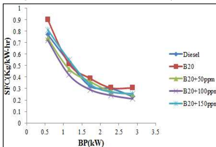
Figure 3. Variation of Specific fuel consumption with B.P
