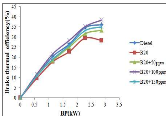
Figure 2. Variation of Brake thermal efficiency with B.P
