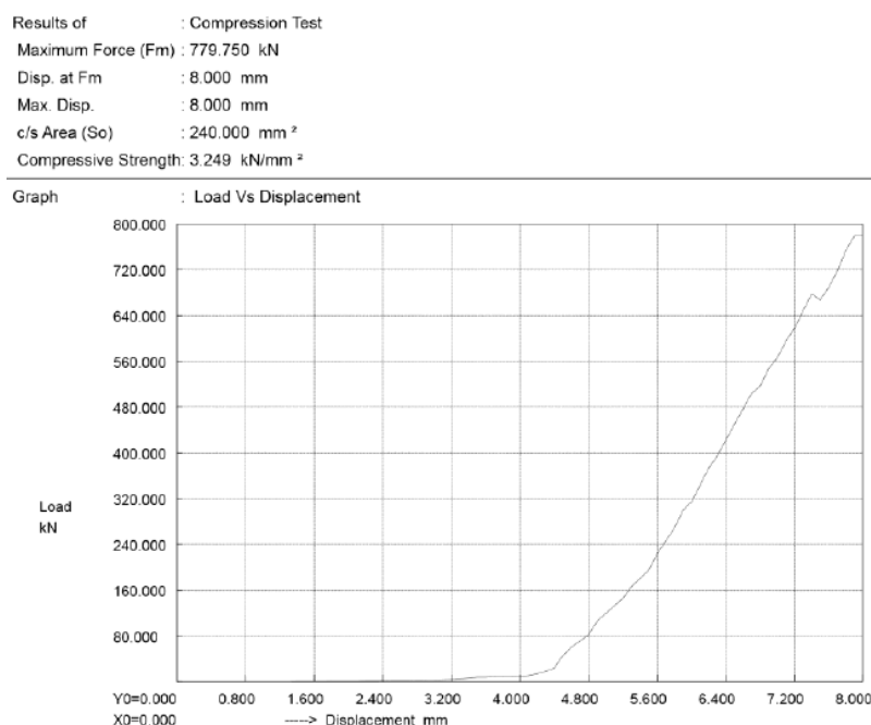
Figure 3: Compression Test Results
