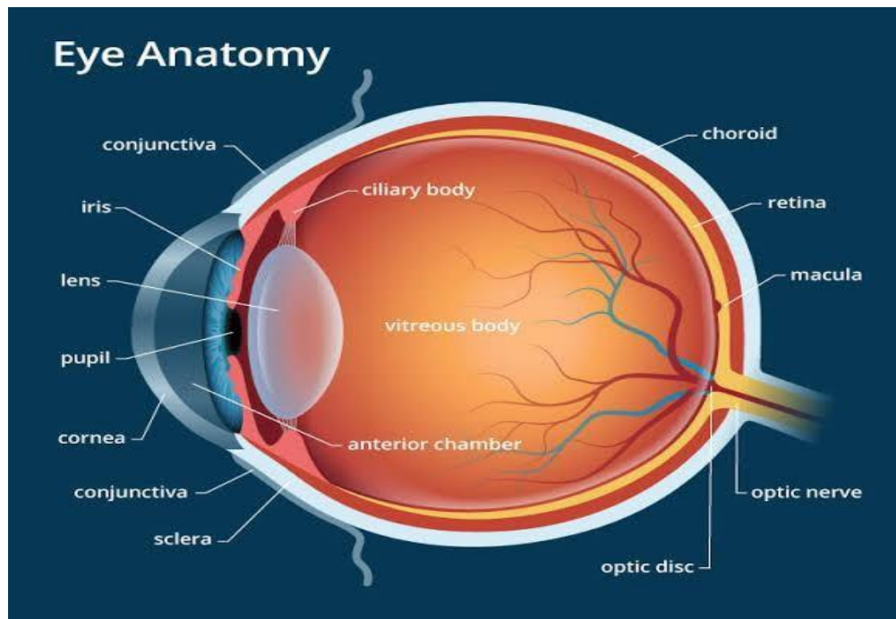
fig.1 Eye anatomy
