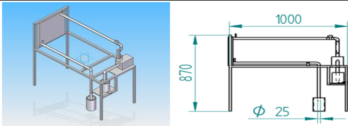
Figure 1: Isometric & Front View of the test rig model
